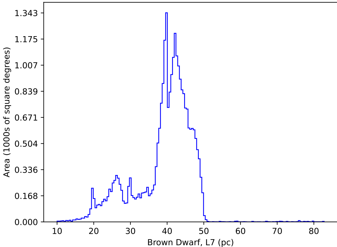
early_ss_template_fpextra3.0_v3.4_10yrs : Brown Dwarf, L7
