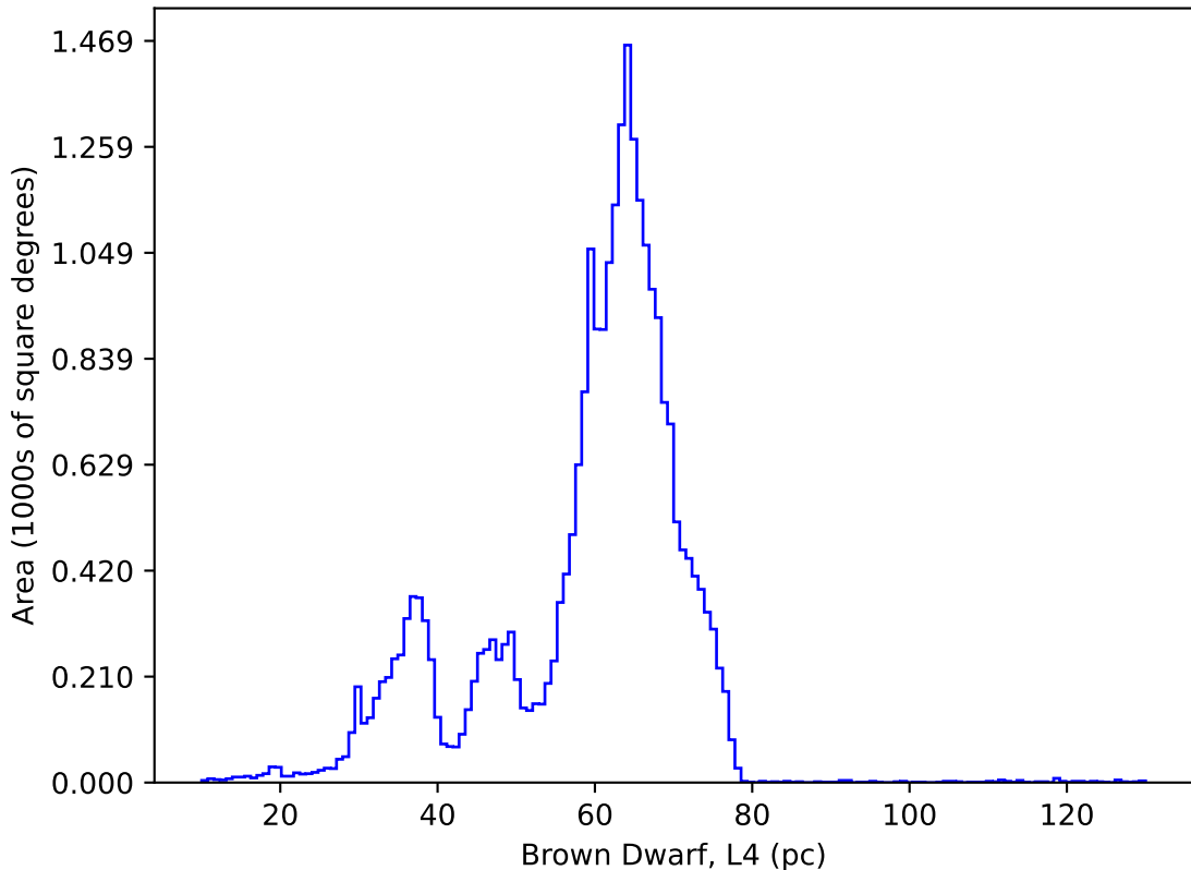
early_ss_template_fpextra3.0_v3.4_10yrs : Brown Dwarf, L4
