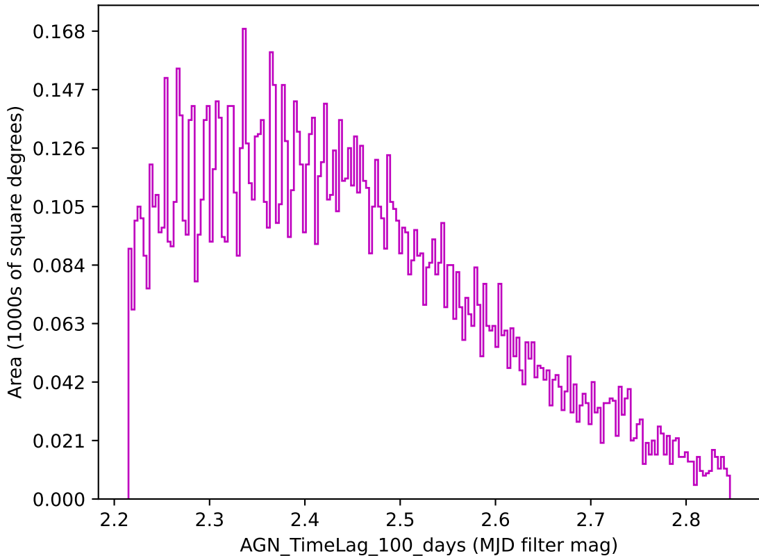
early_ss_template_fpextra3.0_v3.4_10yrs z band: AGN_TimeLag_100_days
