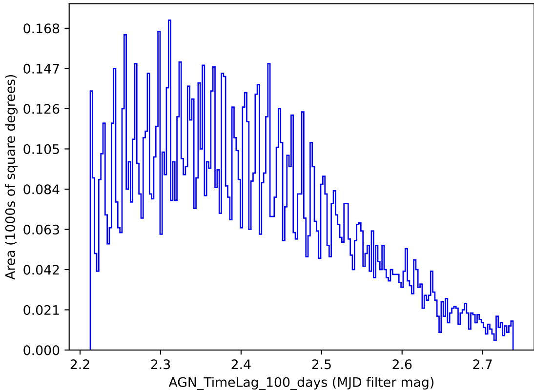
early_ss_template_fpextra3.0_v3.4_10yrs y band: AGN_TimeLag_100_days
