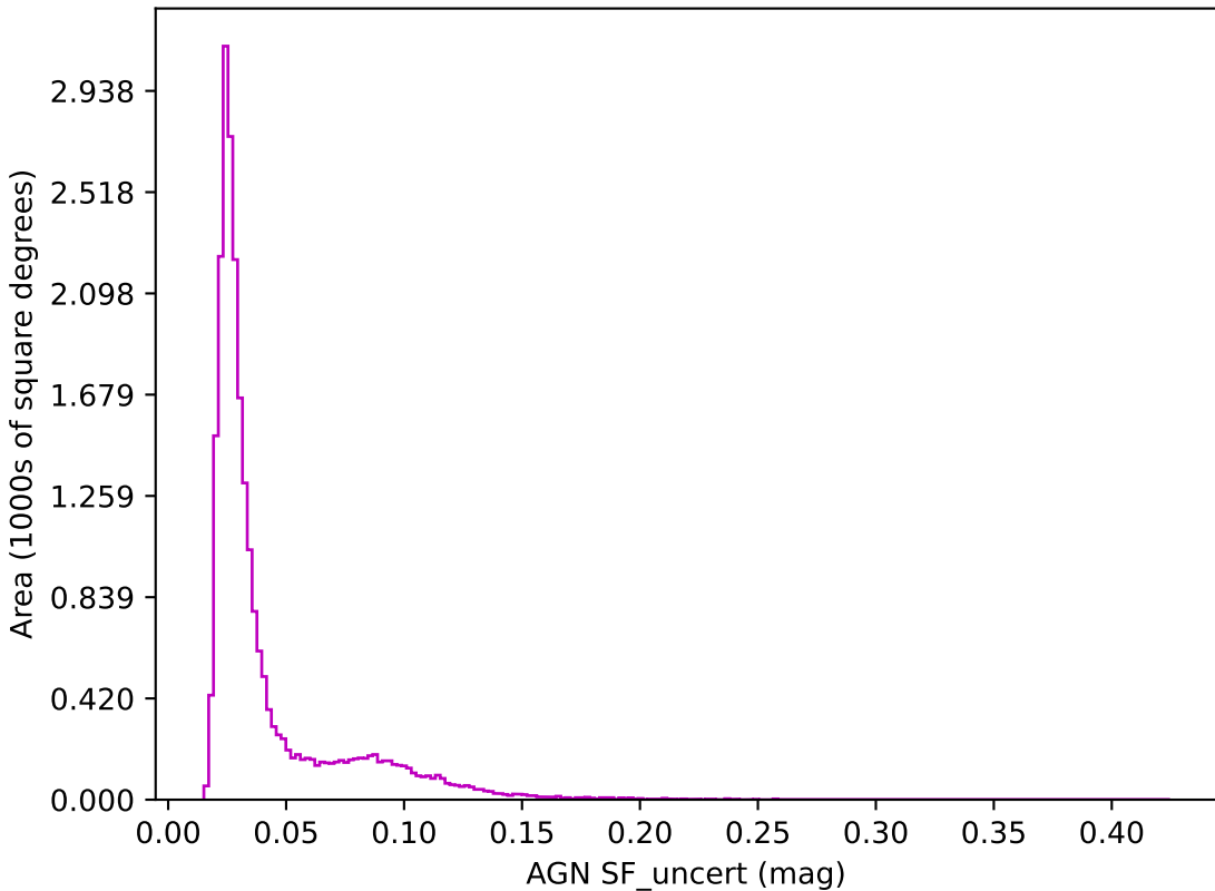
early_ss_template_fpextra3.0_v3.4_10yrs z band: AGN SF_uncert
