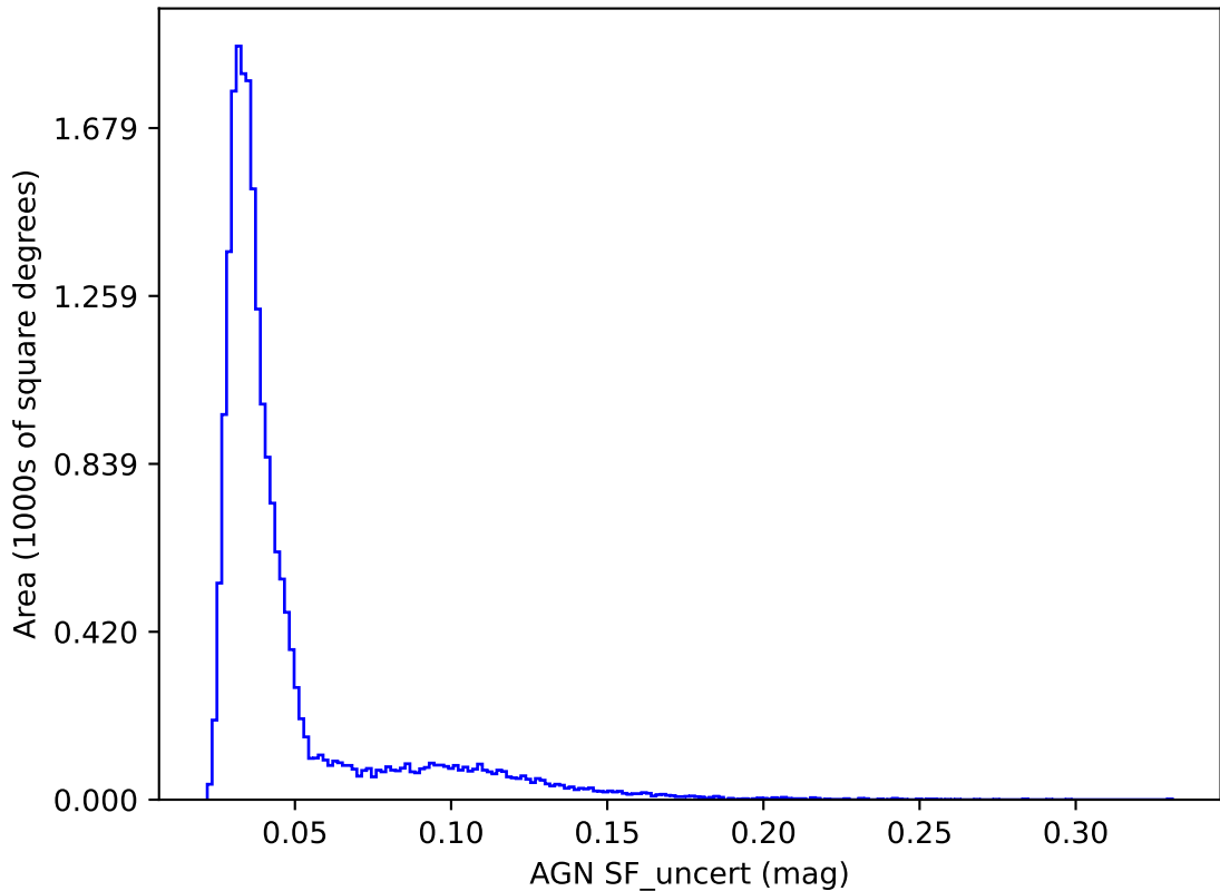
early_ss_template_fpextra3.0_v3.4_10yrs y band: AGN SF_uncert
