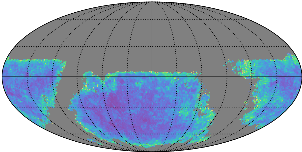
early_ss_template_fpextra3.0_v3.4_10yrs u band: AGN SF_uncert
