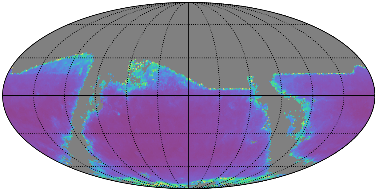
early_ss_template_fpextra3.0_v3.4_10yrs r band: AGN SF_uncert
