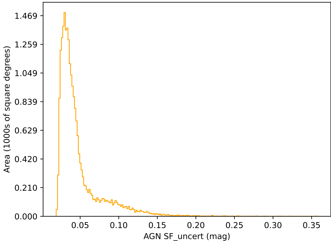
early_ss_template_fpextra3.0_v3.4_10yrs r band: AGN SF_uncert
