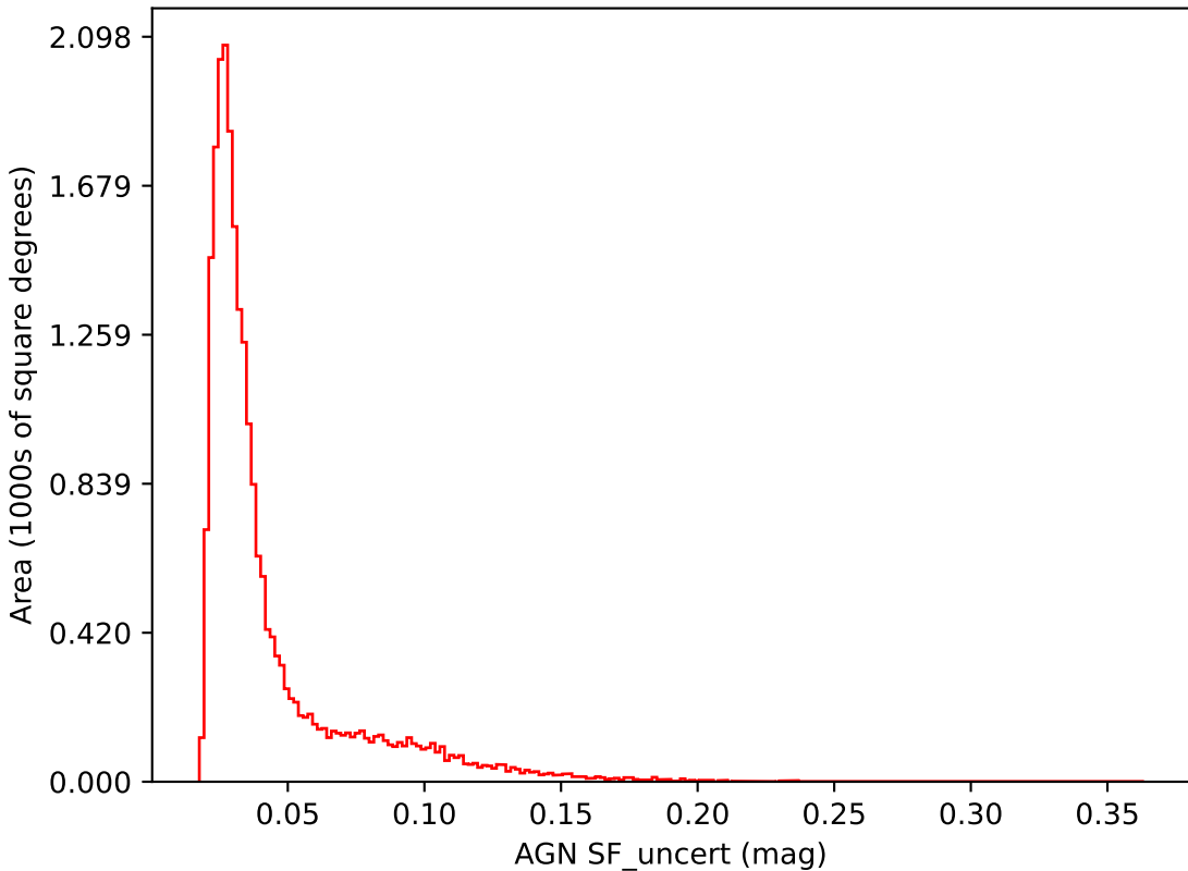
early_ss_template_fpextra3.0_v3.4_10yrs i band: AGN SF_uncert
