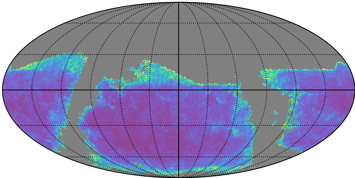
early_ss_template_fpextra3.0_v3.4_10yrs g band: AGN SF_uncert
