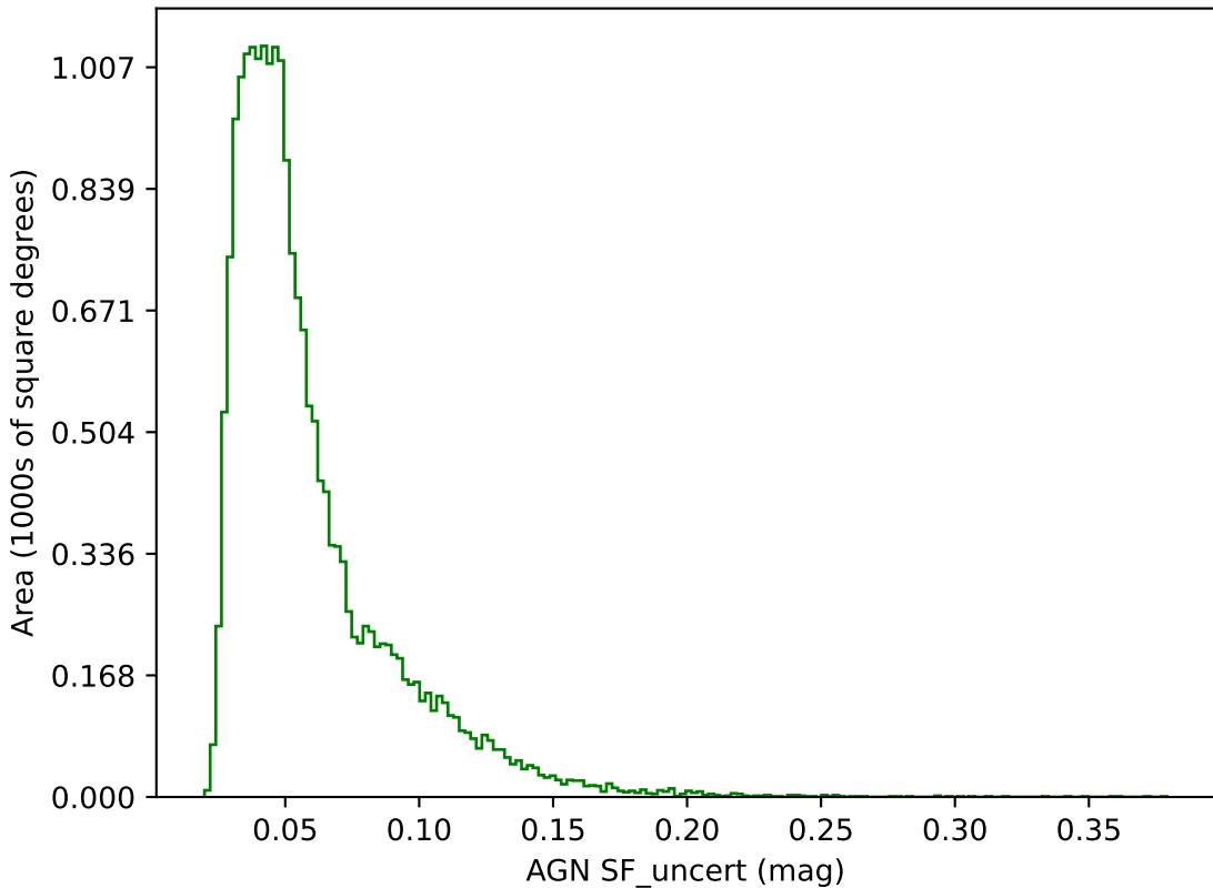
early_ss_template_fpextra3.0_v3.4_10yrs g band: AGN SF_uncert
