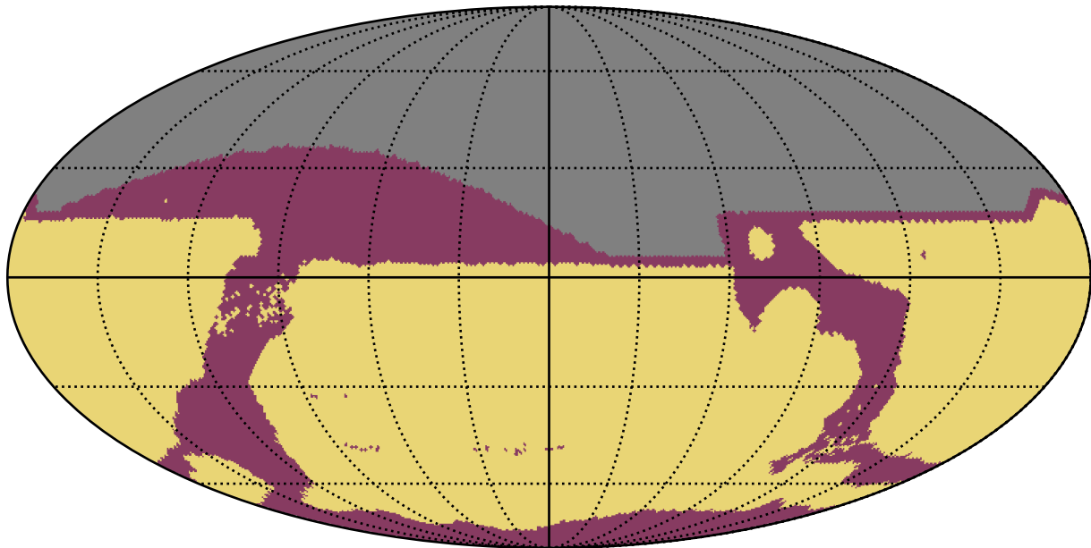
early_ss_template_fpextra3.0_v3.4_10yrs All sky: RapidRevisits
