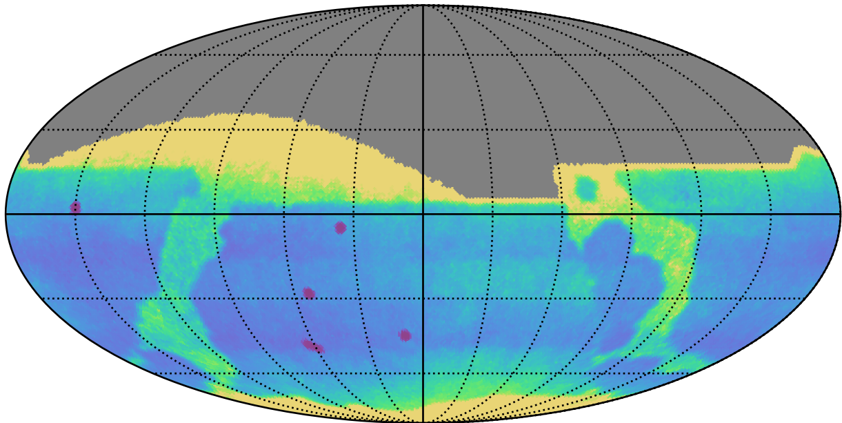
early_ss_template_fpextra3.0_v3.4_10yrs All sky: Proper Motion Uncert @ 24.0
