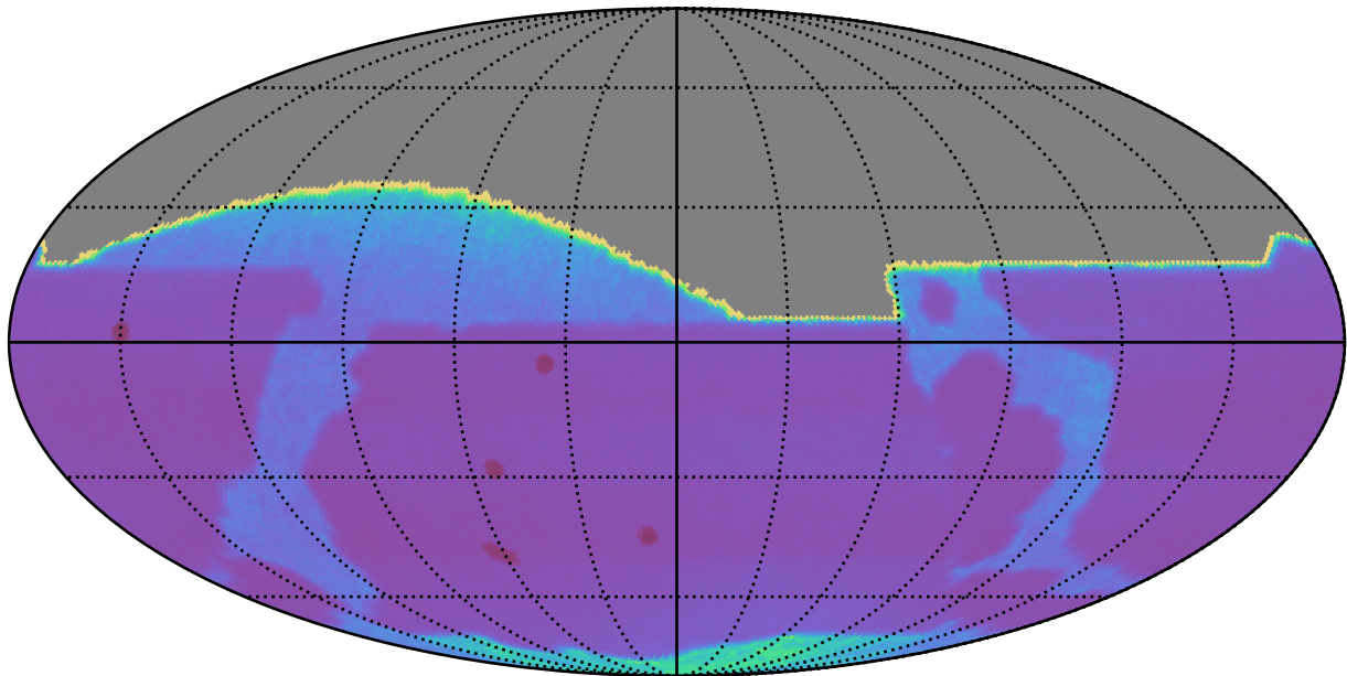
early_ss_template_fpextra3.0_v3.4_10yrs All sky: Proper Motion Uncert @ 20.5
