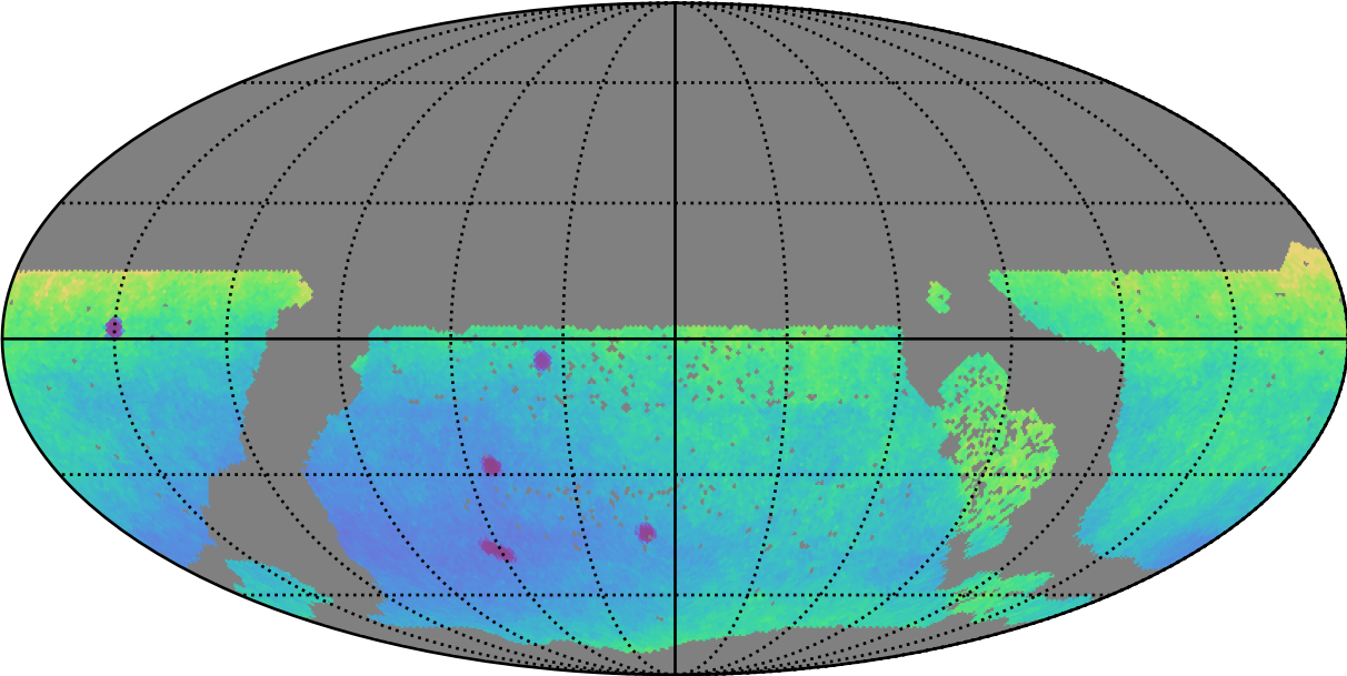
early_ss_template_fpextra3.0_v3.4_10yrs WFD y band only: Parallax Uncert @ 21.3
