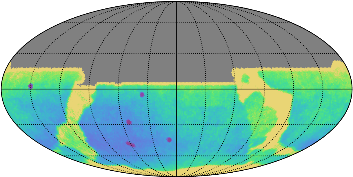
early_ss_template_fpextra3.0_v3.4_10yrs All sky y band only: Parallax Uncert @ 21.3
