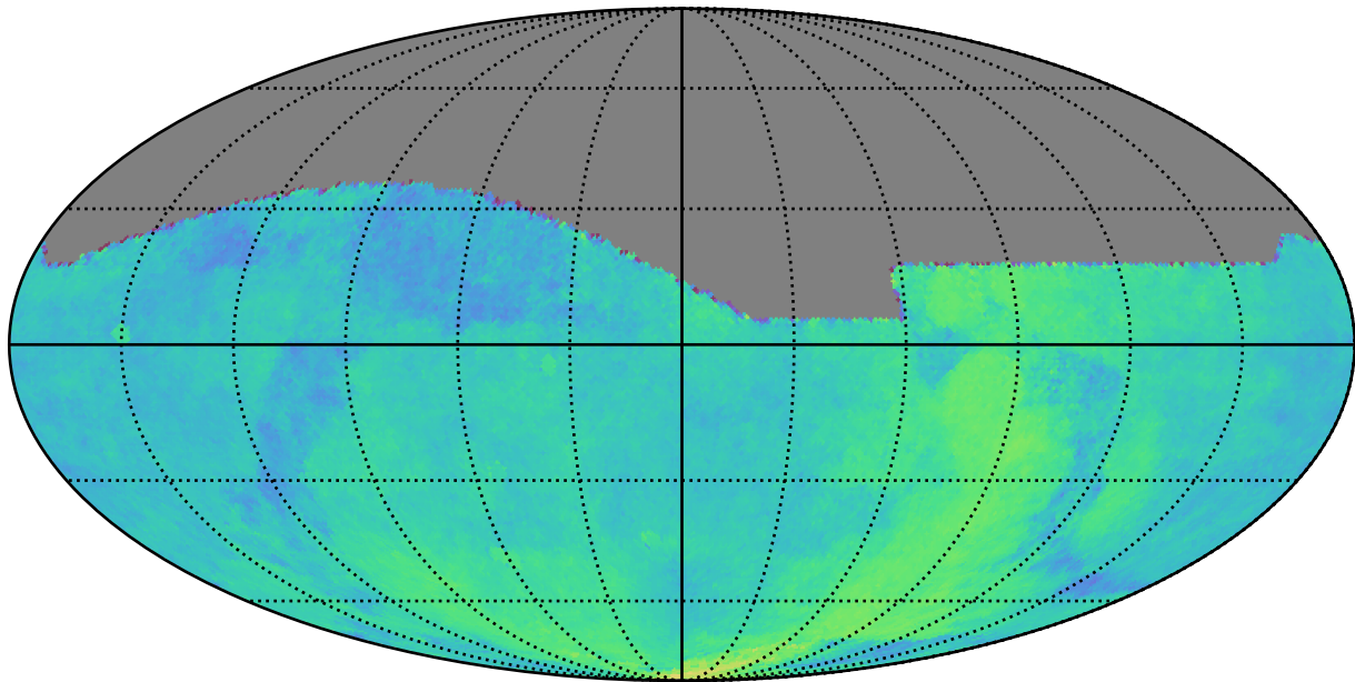
early_ss_template_fpextra3.0_v3.4_10yrs All sky: Parallax Coverage @ 24.0
