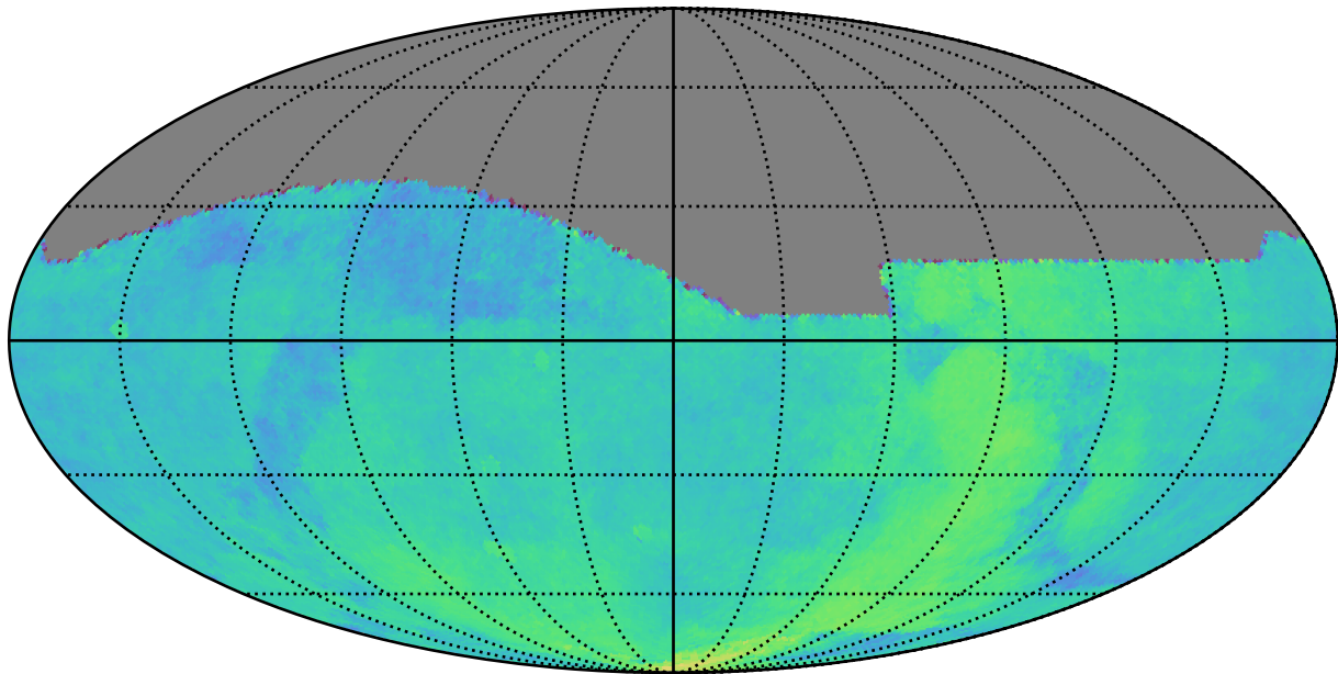
early_ss_template_fpextra3.0_v3.4_10yrs All sky: Parallax Coverage @ 22.4
