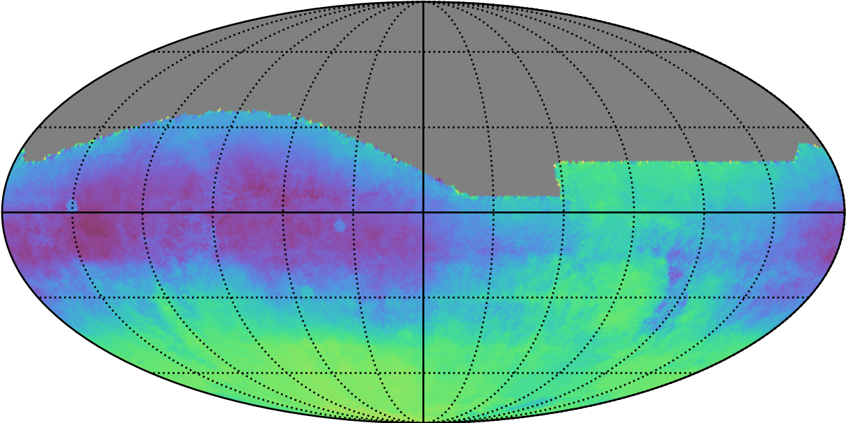
early_ss_template_fpextra3.0_v3.4_10yrs All sky: Parallax-DCR degeneracy @ 24.0
