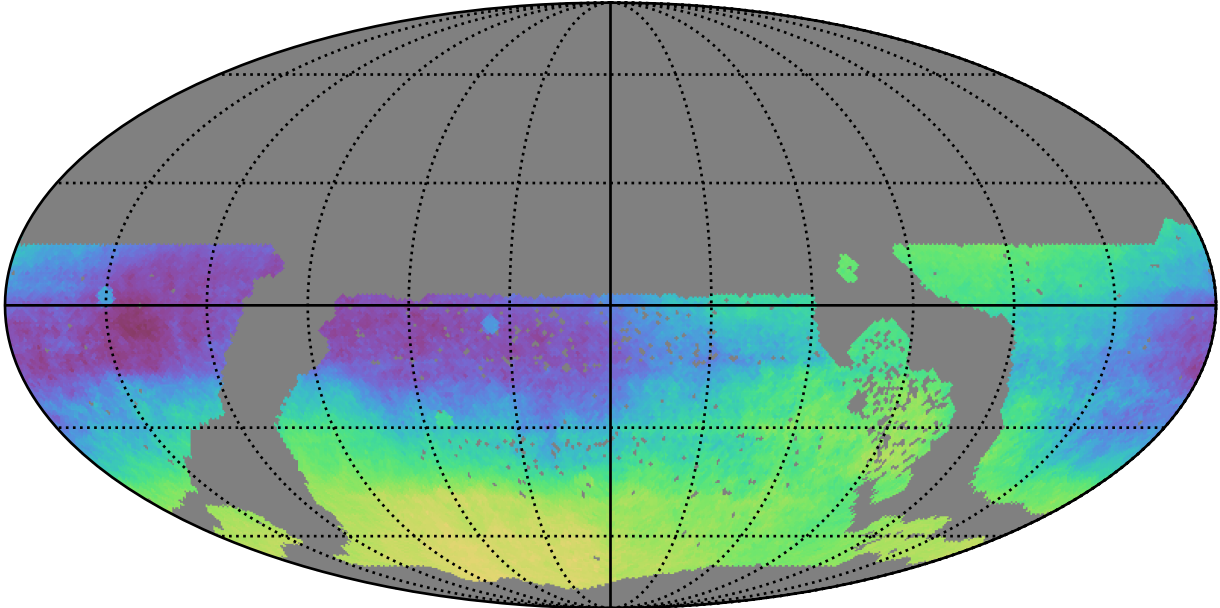
early_ss_template_fpextra3.0_v3.4_10yrs WFD: Parallax-DCR degeneracy @ 22.4
