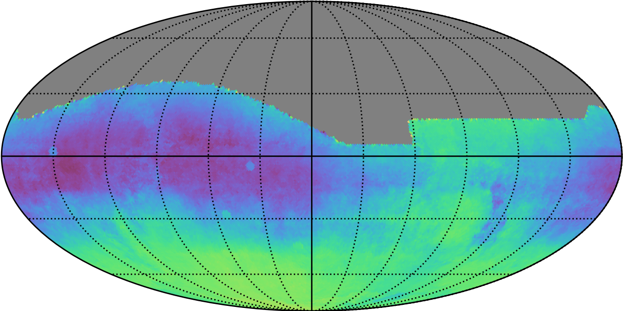
early_ss_template_fpextra3.0_v3.4_10yrs All sky: Parallax-DCR degeneracy @ 22.4
