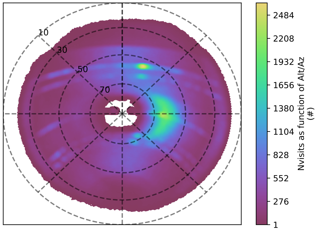
early_ss_template_fpextra3.0_v3.4_10yrs z band: Nvisits as function of Alt/Az
