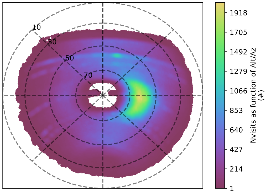
early_ss_template_fpextra3.0_v3.4_10yrs y band: Nvisits as function of Alt/Az
