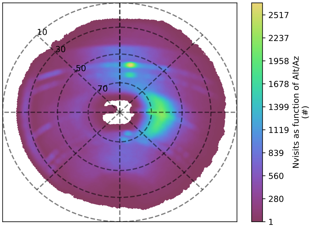
early_ss_template_fpextra3.0_v3.4_10yrs r band: Nvisits as function of Alt/Az
