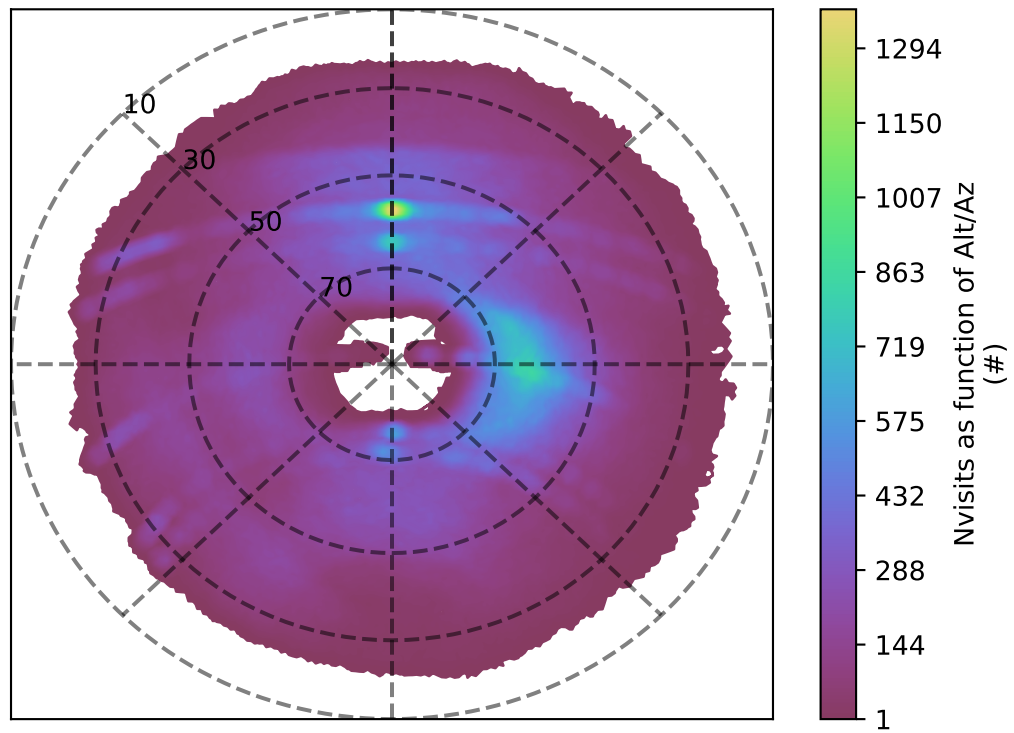
early_ss_template_fpextra3.0_v3.4_10yrs g band: Nvisits as function of Alt/Az
