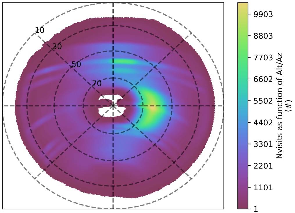
early_ss_template_fpextra3.0_v3.4_10yrs all bands: Nvisits as function of Alt/Az
