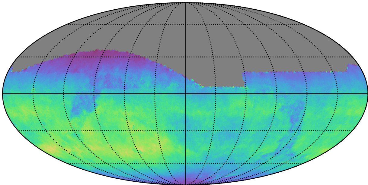
early_ss_template_fpextra3.0_v3.4_10yrs All sky z band: Normalized Teff
