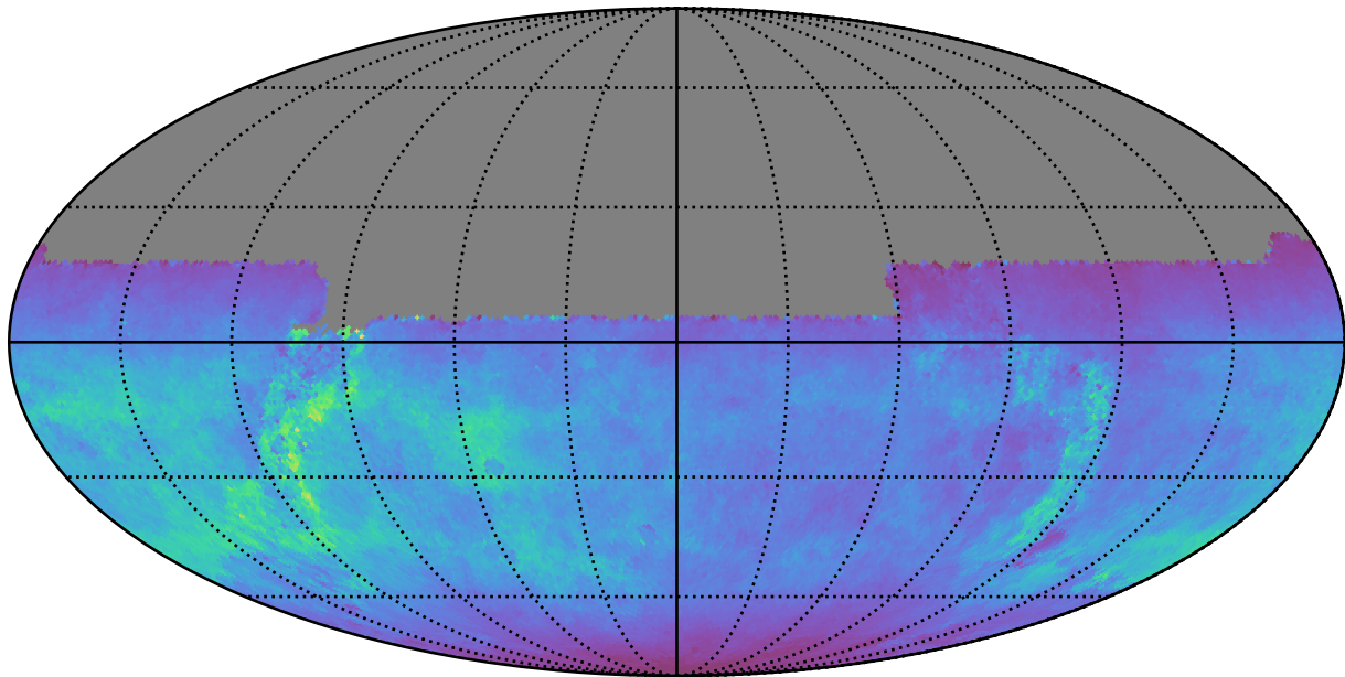
early_ss_template_fpextra3.0_v3.4_10yrs All sky u band: Normalized Teff
