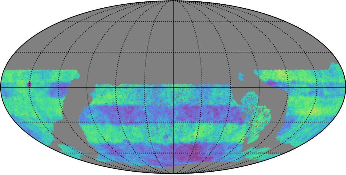
early_ss_template_fpextra3.0_v3.4_10yrs WFD: Normalized Proper Motion Uncert @ 24.0
