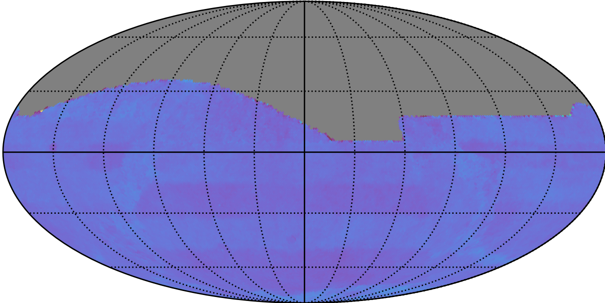
early_ss_template_fpextra3.0_v3.4_10yrs All sky: Normalized Proper Motion Uncert @ 24.0
