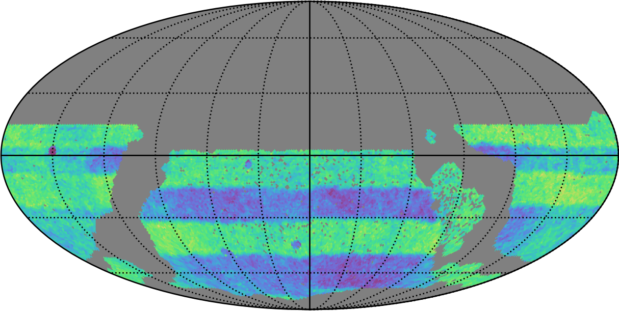
early_ss_template_fpextra3.0_v3.4_10yrs WFD: Normalized Proper Motion Uncert @ 20.5
