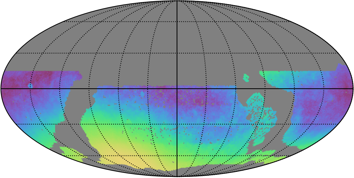
early_ss_template_fpextra3.0_v3.4_10yrs WFD: Normalized Parallax Uncert @ 24.0
