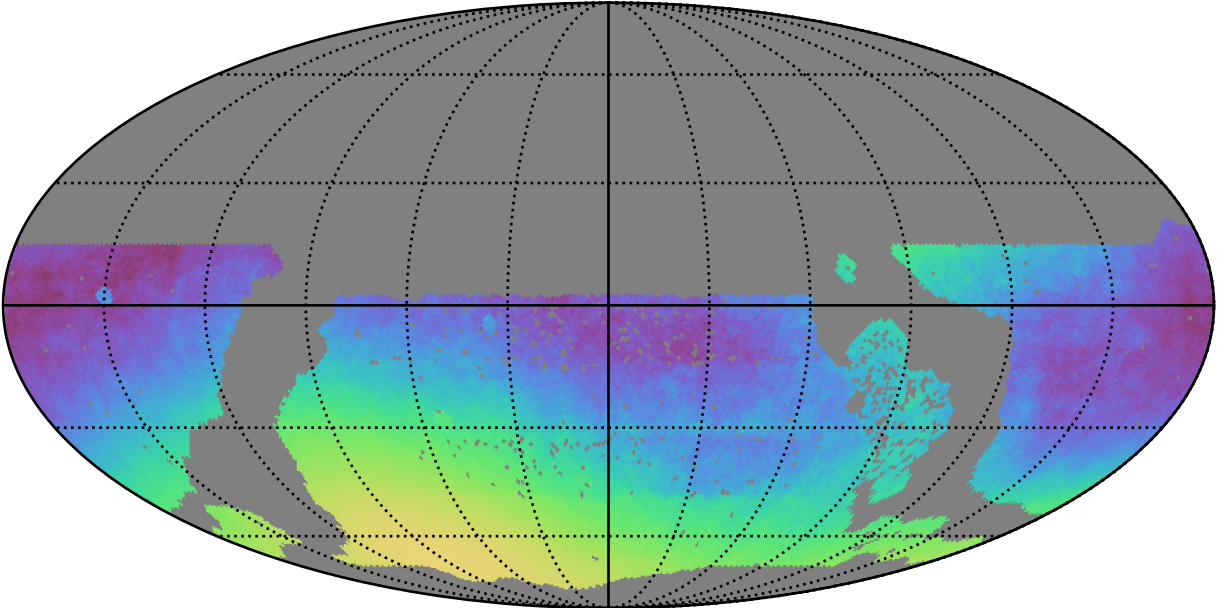
early_ss_template_fpextra3.0_v3.4_10yrs WFD: Normalized Parallax Uncert @ 22.4
