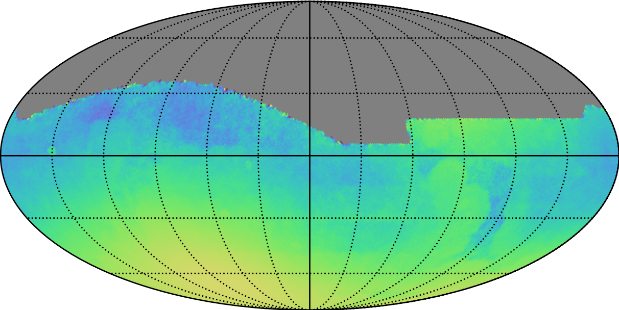
early_ss_template_fpextra3.0_v3.4_10yrs All sky: Normalized Parallax Uncert @ 22.4
