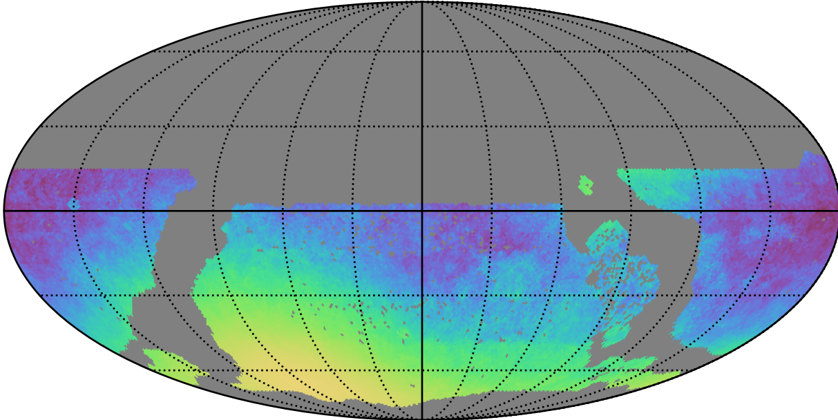
early_ss_template_fpextra3.0_v3.4_10yrs WFD y band only: Normalized Parallax Uncert @ 21.3
