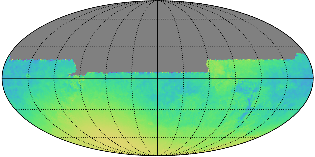
early_ss_template_fpextra3.0_v3.4_10yrs All sky y band only: Normalized Parallax Uncert @ 21.3
