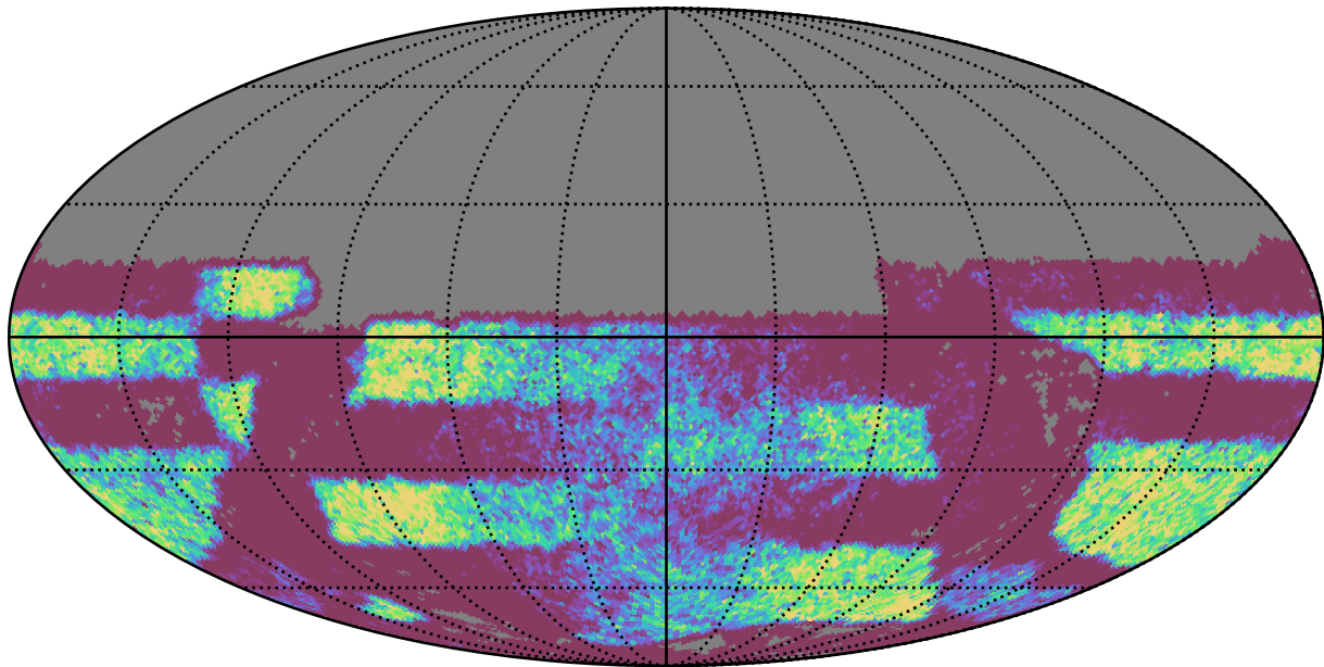
early_ss_template_fpextra3.0_v3.4_10yrs Yr 3-4 y band: NVisits
