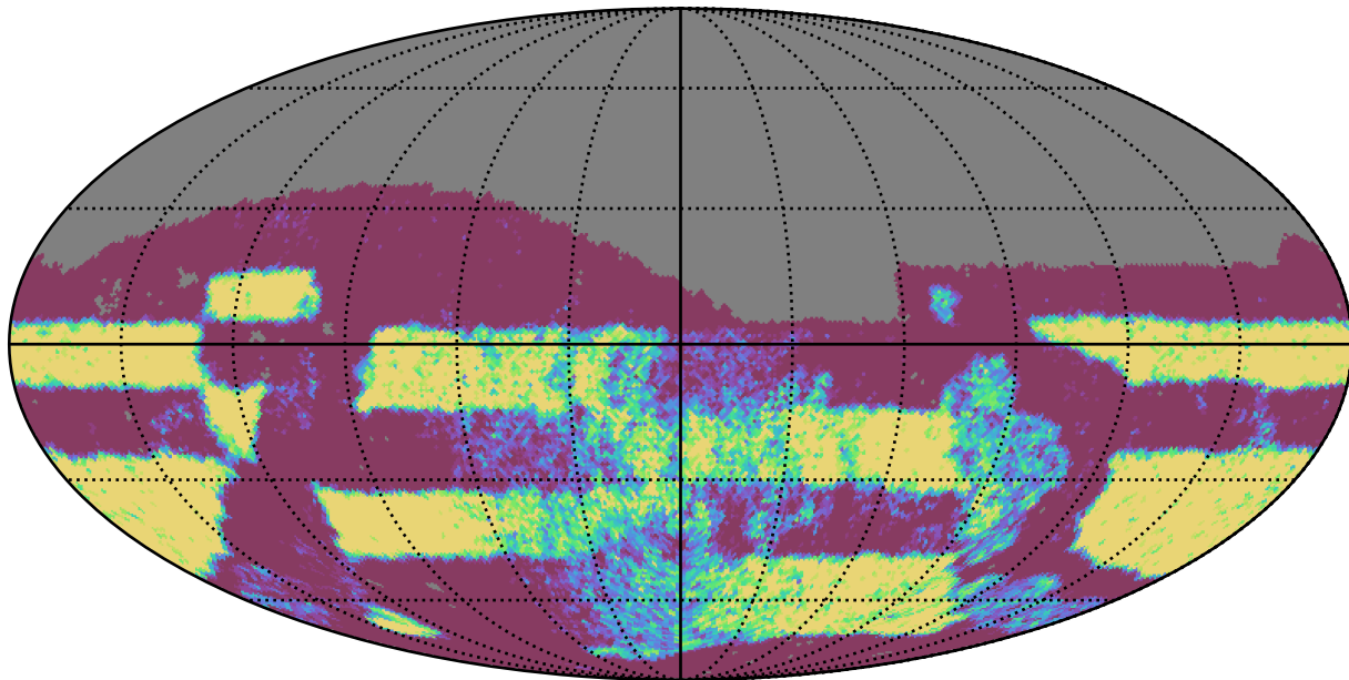
early_ss_template_fpextra3.0_v3.4_10yrs Yr 3-4 i band: NVisits
