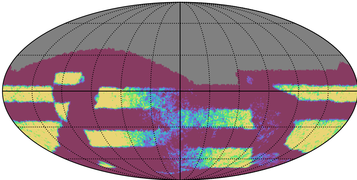
early_ss_template_fpextra3.0_v3.4_10yrs Yr 3-4 all bands: NVisits
