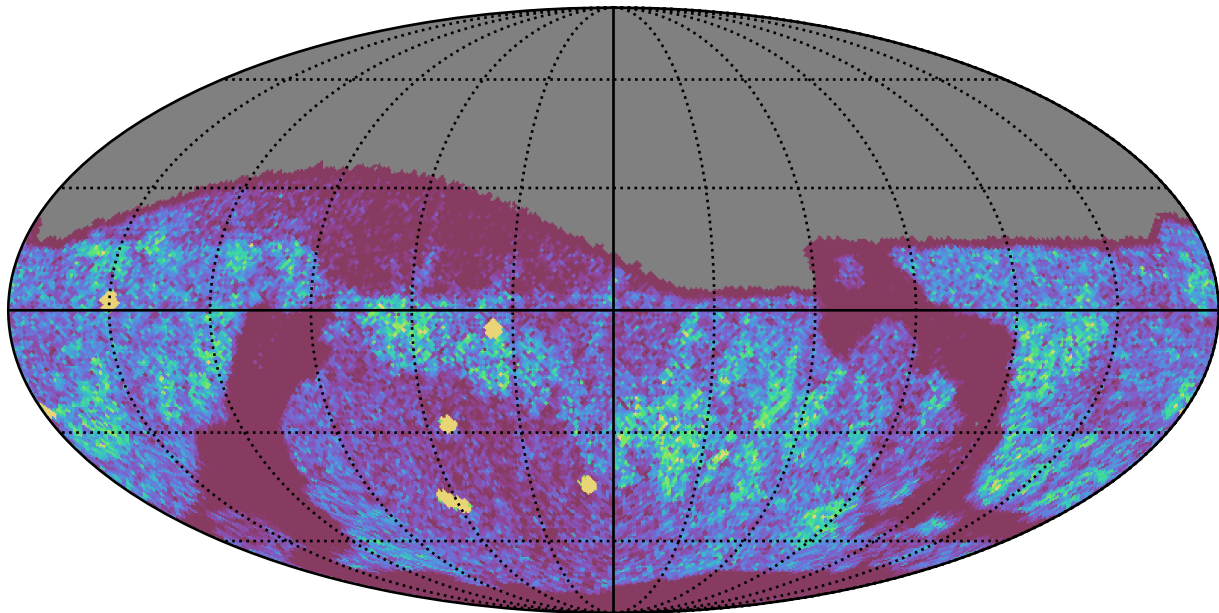
early_ss_template_fpextra3.0_v3.4_10yrs Yr 1 z band: NVisits
