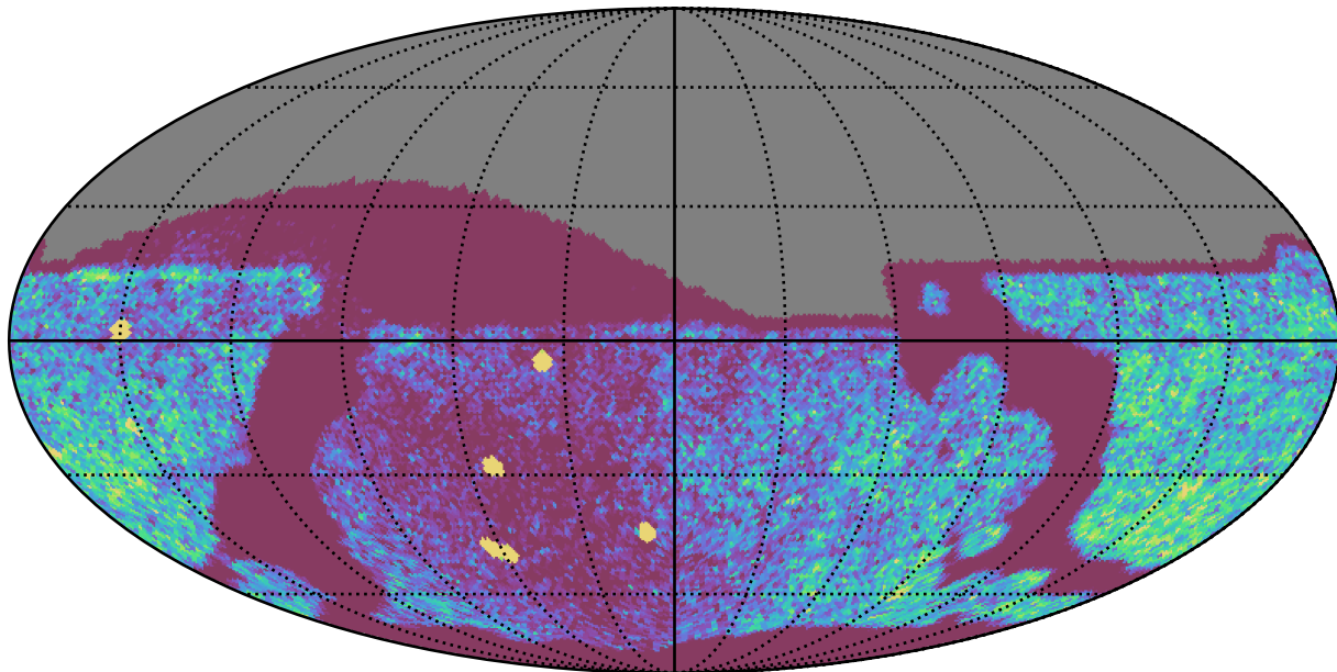
early_ss_template_fpextra3.0_v3.4_10yrs Yr 1 all bands: NVisits
