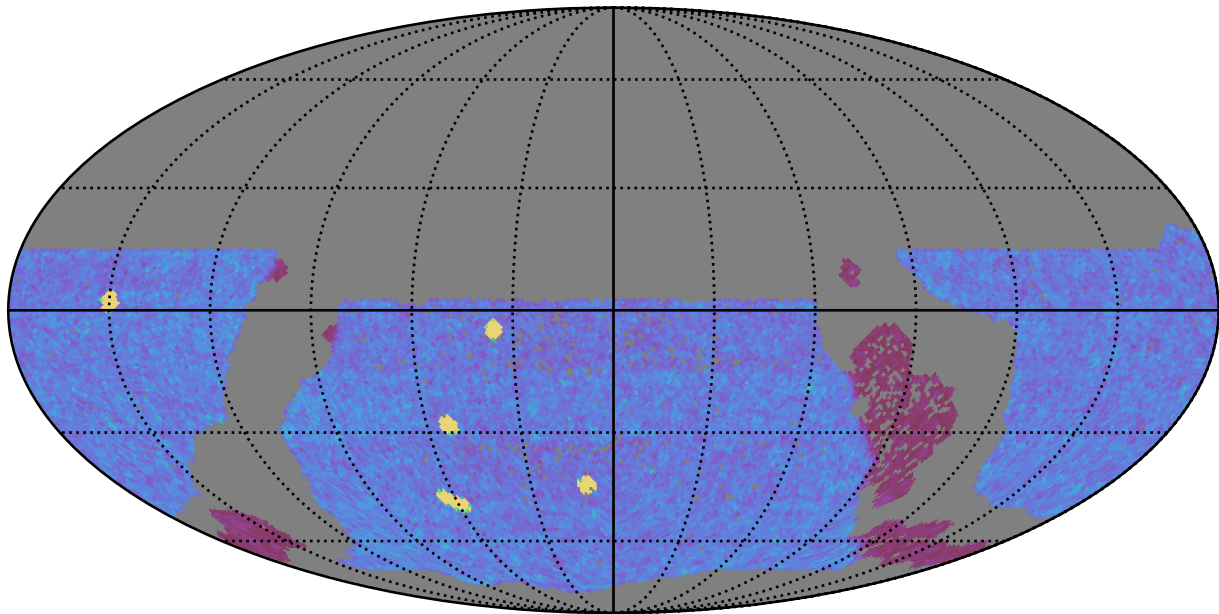
early_ss_template_fpextra3.0_v3.4_10yrs WFD y band: NVisits
