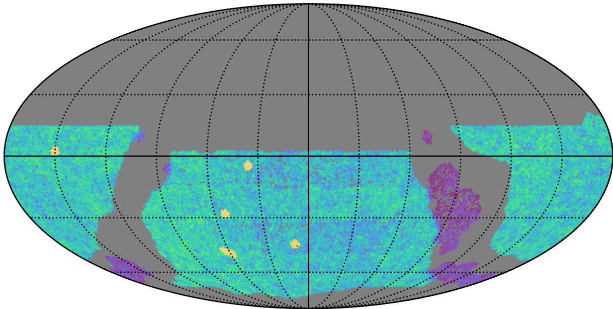
early_ss_template_fpextra3.0_v3.4_10yrs WFD u band: NVisits
