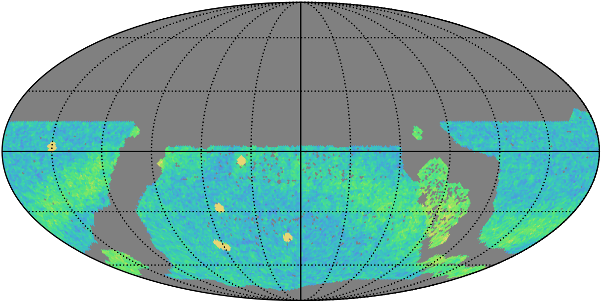
early_ss_template_fpextra3.0_v3.4_10yrs WFD r band: NVisits
