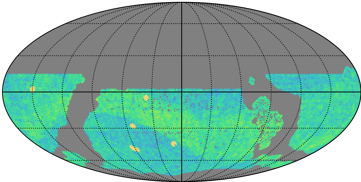
early_ss_template_fpextra3.0_v3.4_10yrs WFD i band: NVisits
