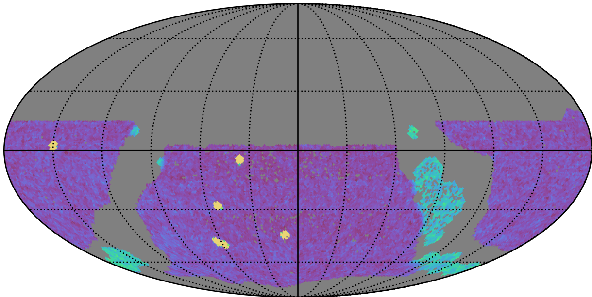
early_ss_template_fpextra3.0_v3.4_10yrs WFD g band: NVisits
