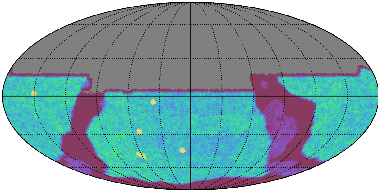
early_ss_template_fpextra3.0_v3.4_10yrs All sky u band: NVisits
