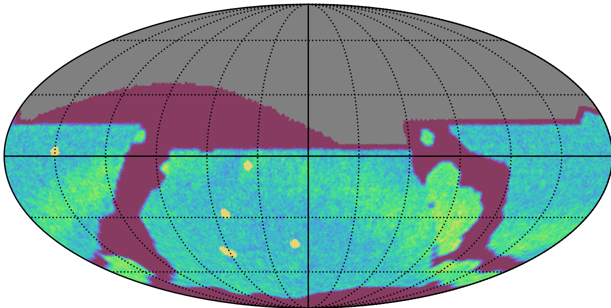
early_ss_template_fpextra3.0_v3.4_10yrs All sky r band: NVisits
