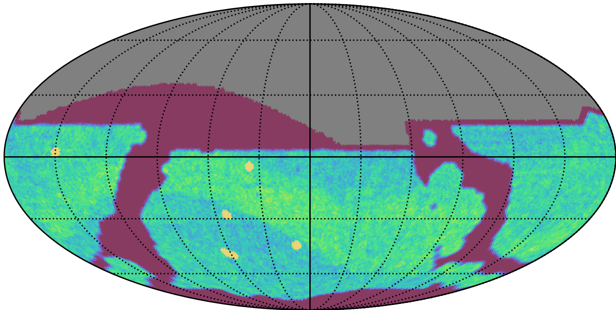
early_ss_template_fpextra3.0_v3.4_10yrs All sky i band: NVisits
